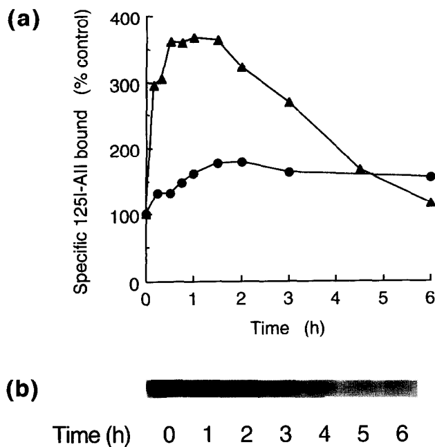
Fig. 1. Time course for the TPA-stimulated increase of [ ^{125} I]AII binding to RIE-1 cells. (a) Cells were incubated with 3 nM (●) or 300 nM TPA (▲) for the indicated times at 37°C. The specific binding of [ ^{125} I]AII was then determined. Each point represents the mean of duplicate determinations. (b) Cells were treated with 300 nM TPA at 37°C for the indicated times. PKC was then detected using immunoblotting as described in the text.
